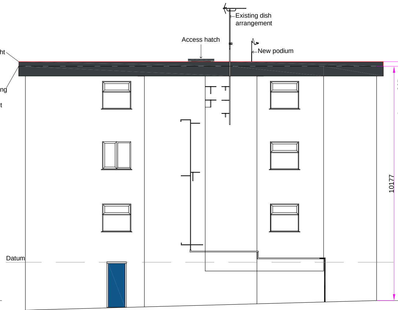
As Proposed West Elevation
