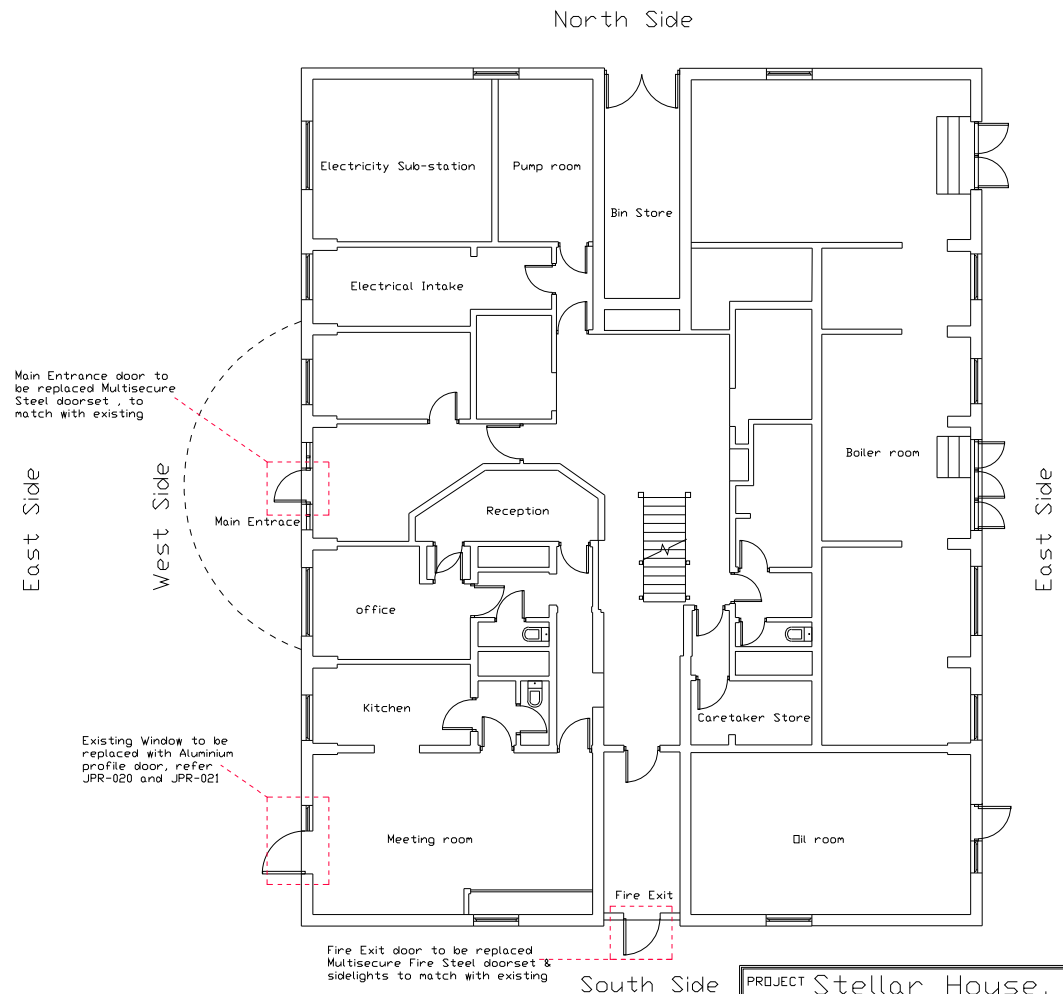
Proposed Ground Floor Layout
