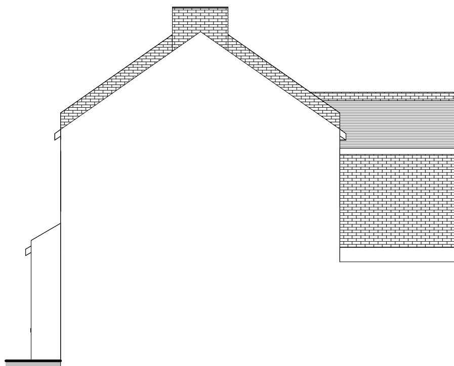
Existing North Elevation 1 : 100
