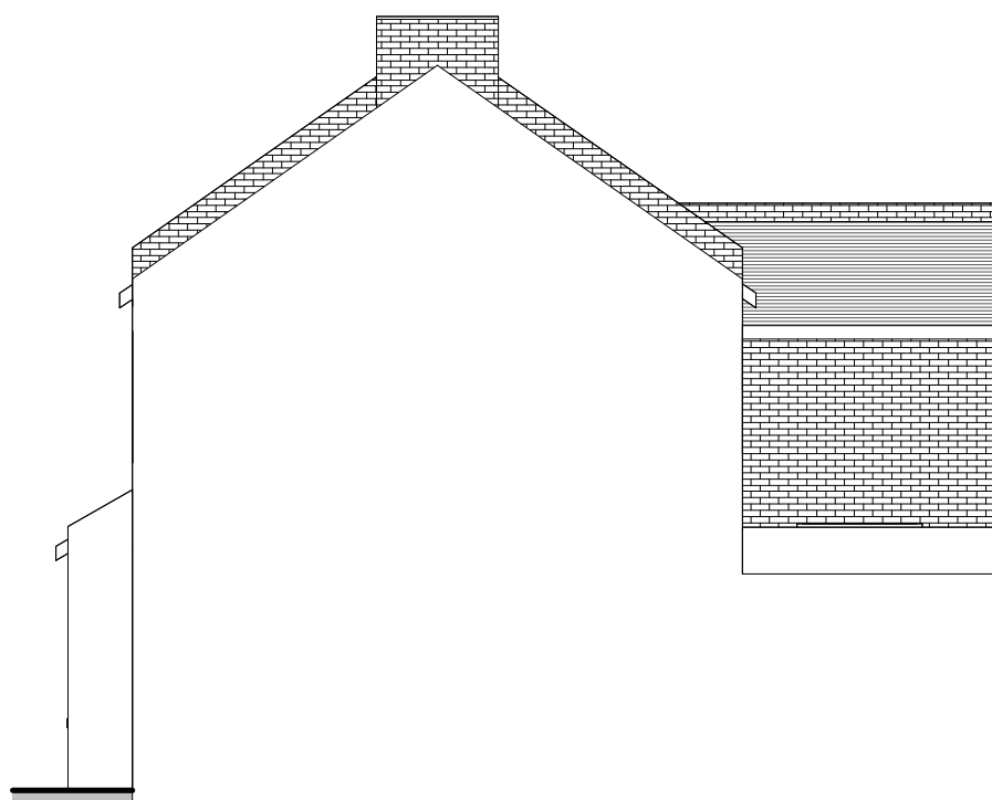
Proposed North Elevation 1 : 100
