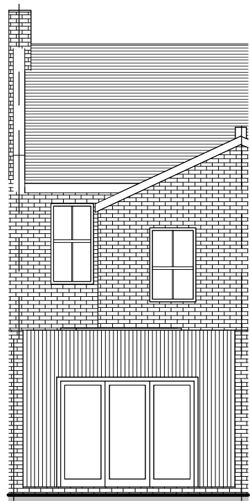
Proposed West Elevation 1 : 100
