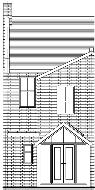
Existing West Elevation 1 : 100
