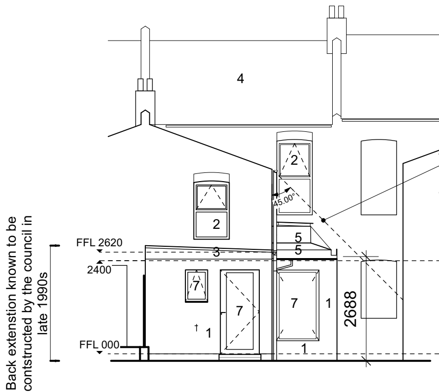
01 054 ELEVATION GABLE
