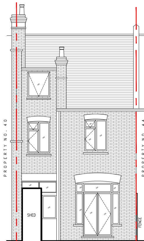
SOUTH ELEVATION
