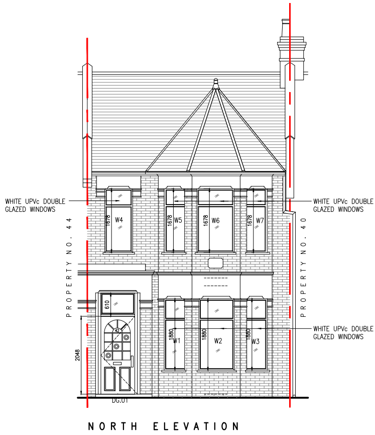
NORTH ELEVATION
