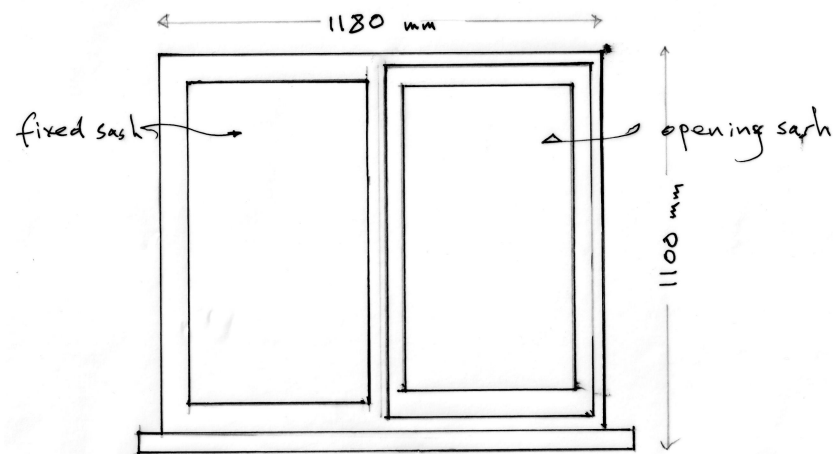
Existing Window 1:20 @ A3
