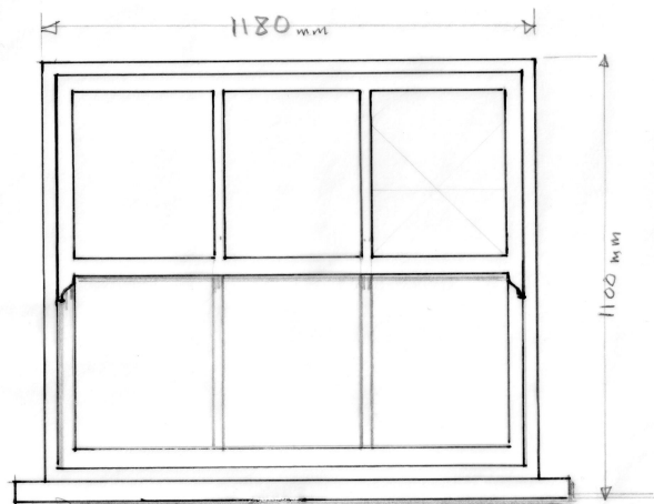
Proposed Window 1:20 @ A3
