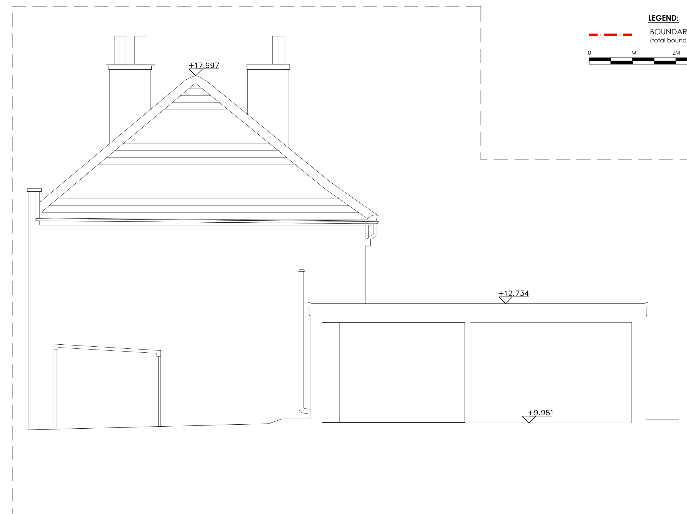
111 C EXISTING SIDE ELEVATION SCALE 1:50 @ A1
