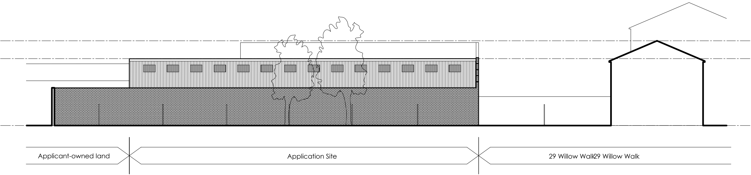
2 East Elevation
