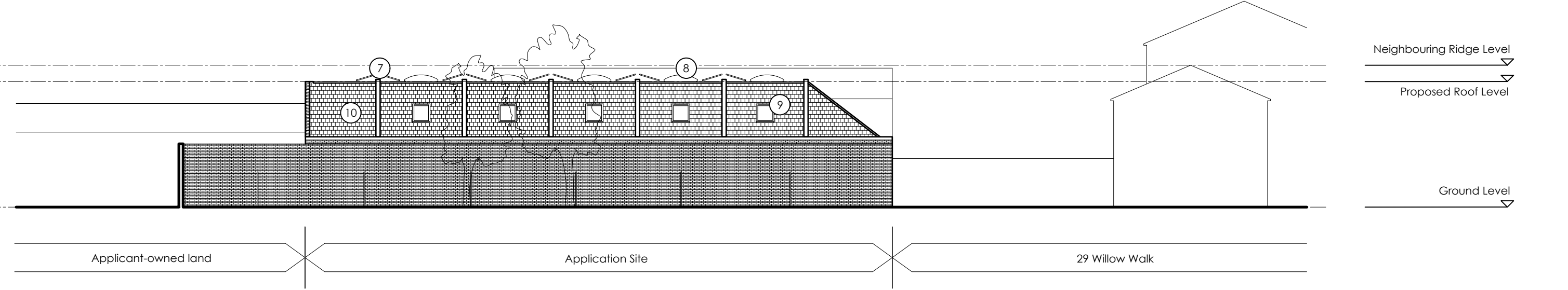
2 Proposed East Elevation
