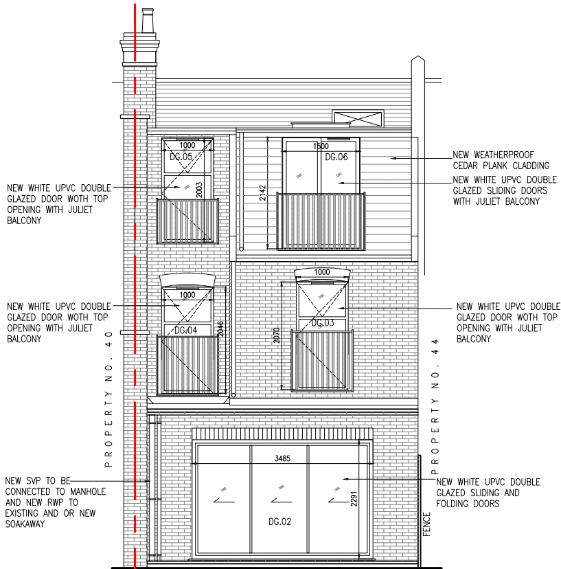
SOUTH ELEVATION
