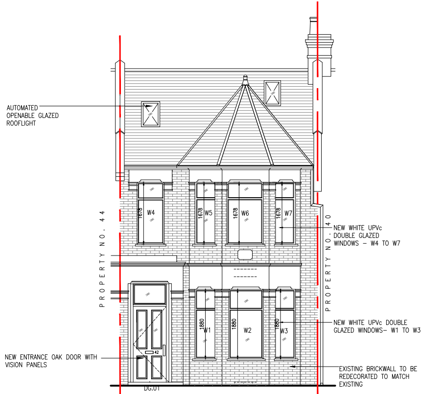
NORTH ELEVATION
