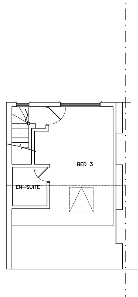
EXISTING LOFT FLOOR PLAN
