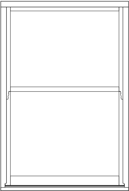
02 - New window with square head Scale 1:20
