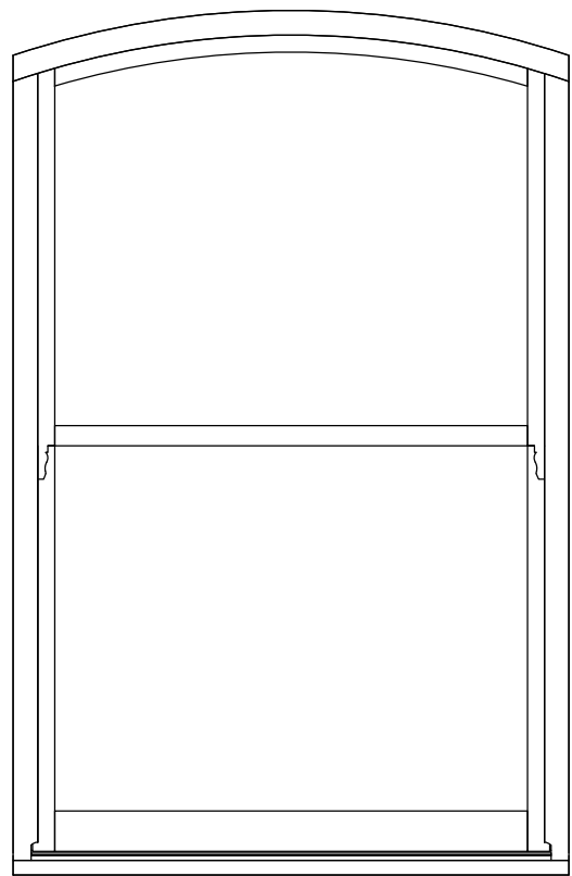
01 - New window with arch head Scale 1:20
