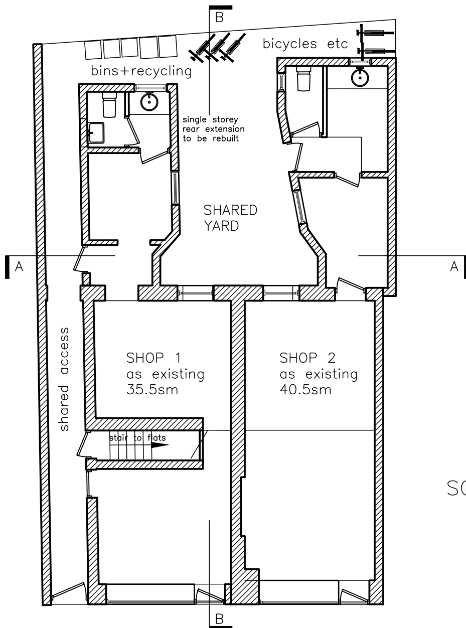
2 FLATS+SHOPS – GROUND
