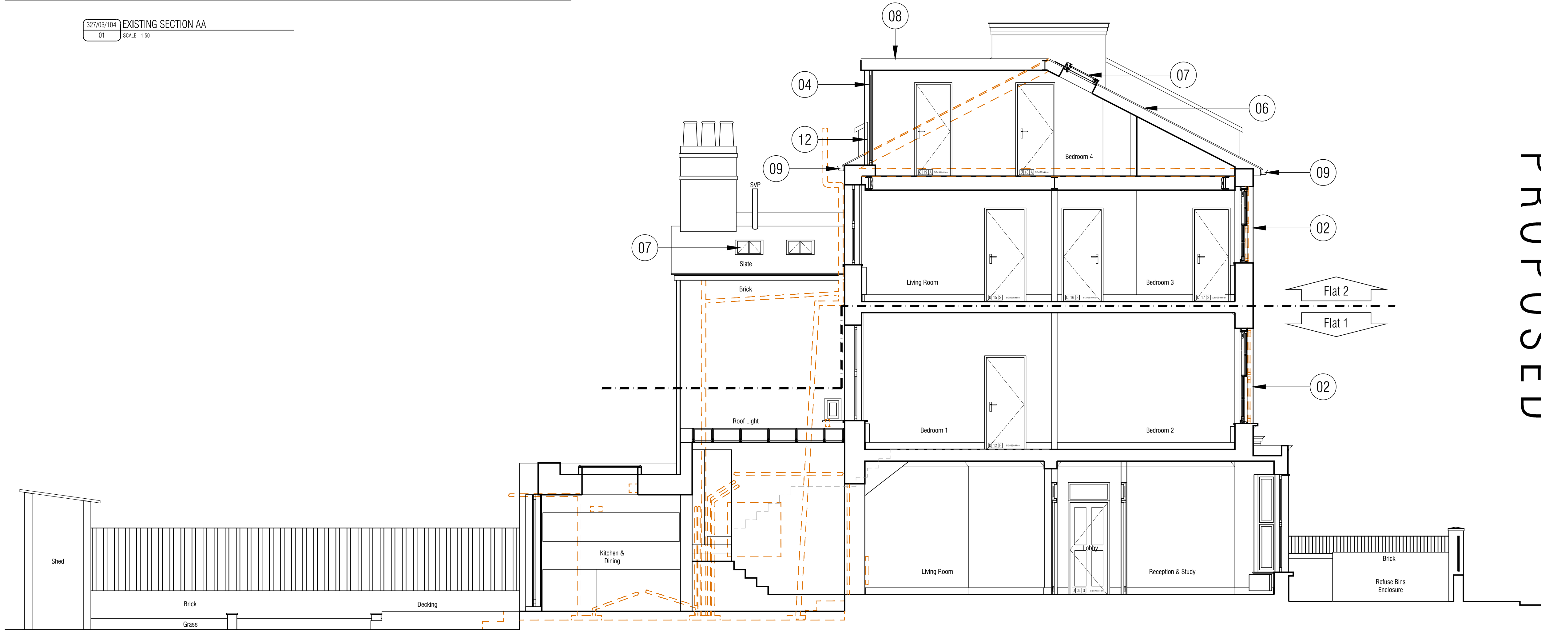
327/03/104 PROPOSED SECTION AA 02 SCALE = 1:50
