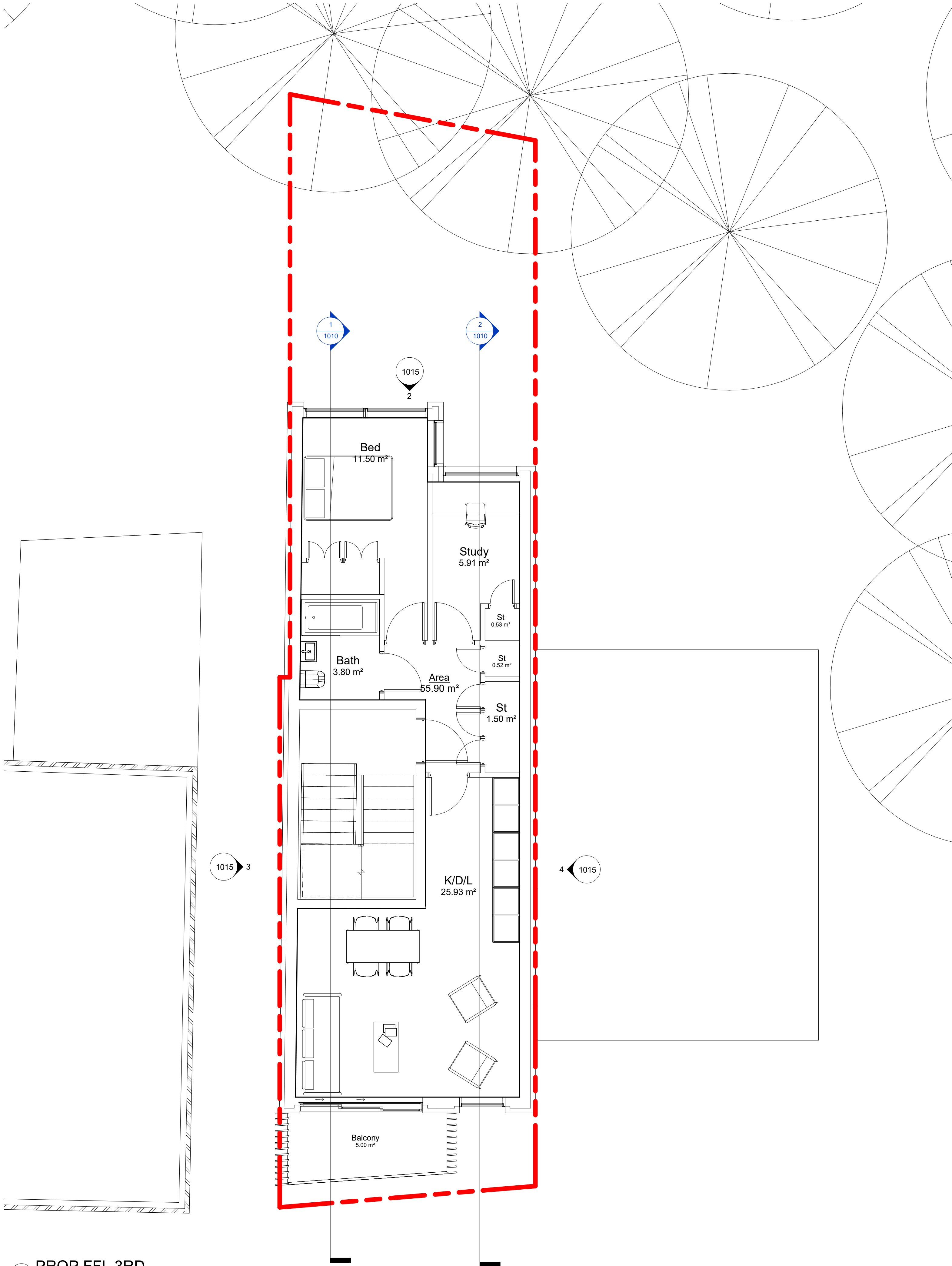
1 PROP FFL 3RD Scale 1 : 50
