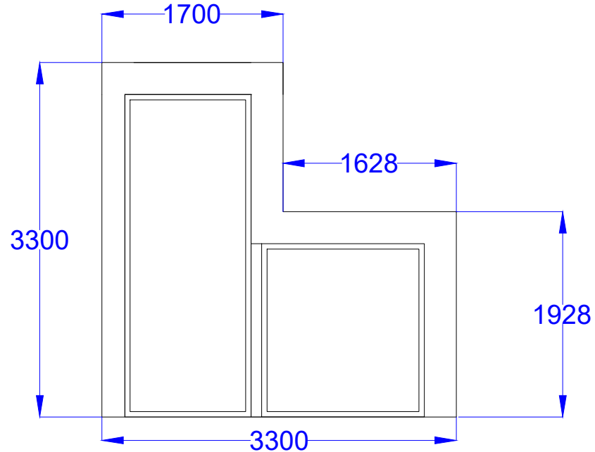
ROOF PLAN
