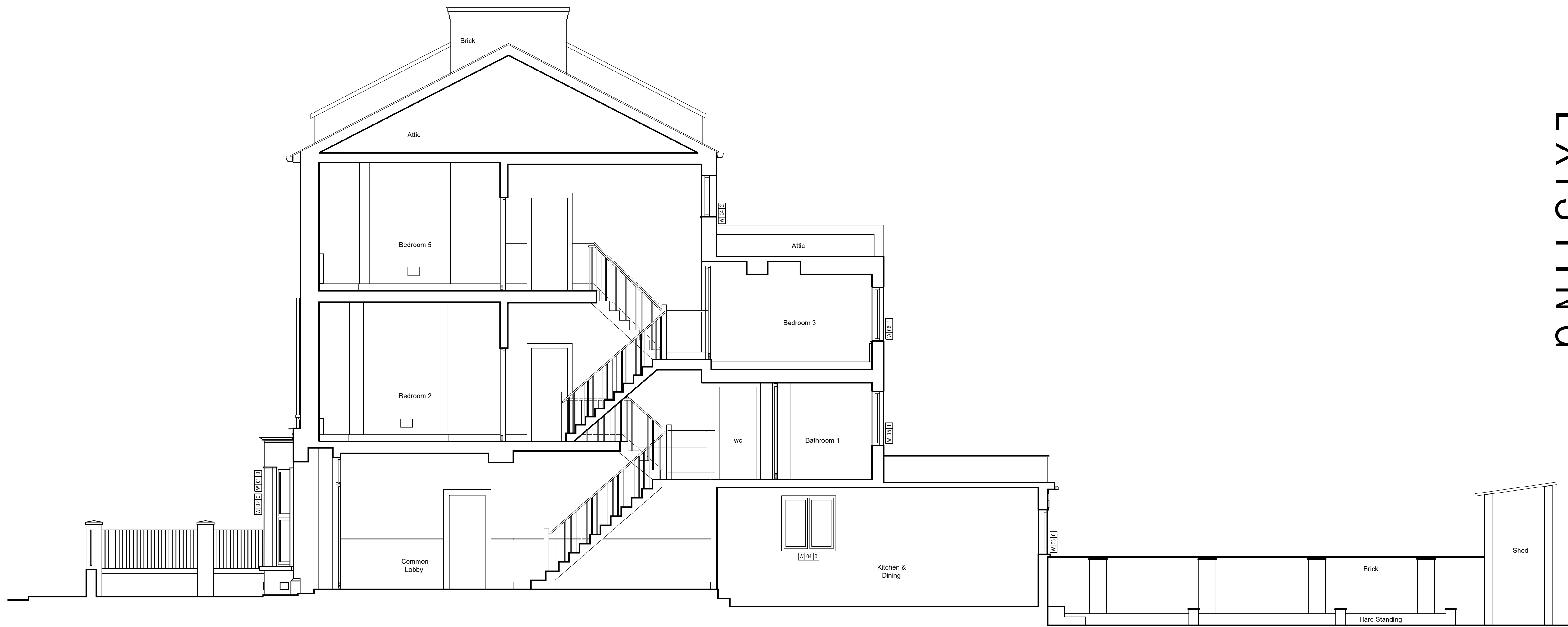
327/03/105 EXISTING SECTION BB 01 SCALE - 1:50
