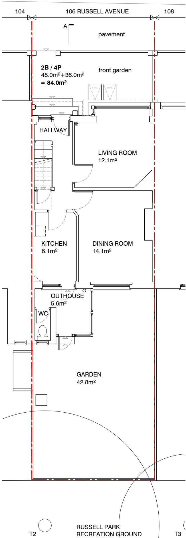
SITE PLAN / GROUND FLOOR
