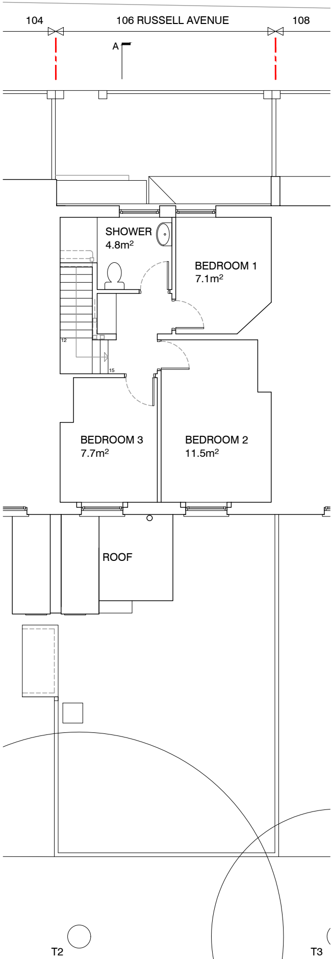
FIRST FLOOR
