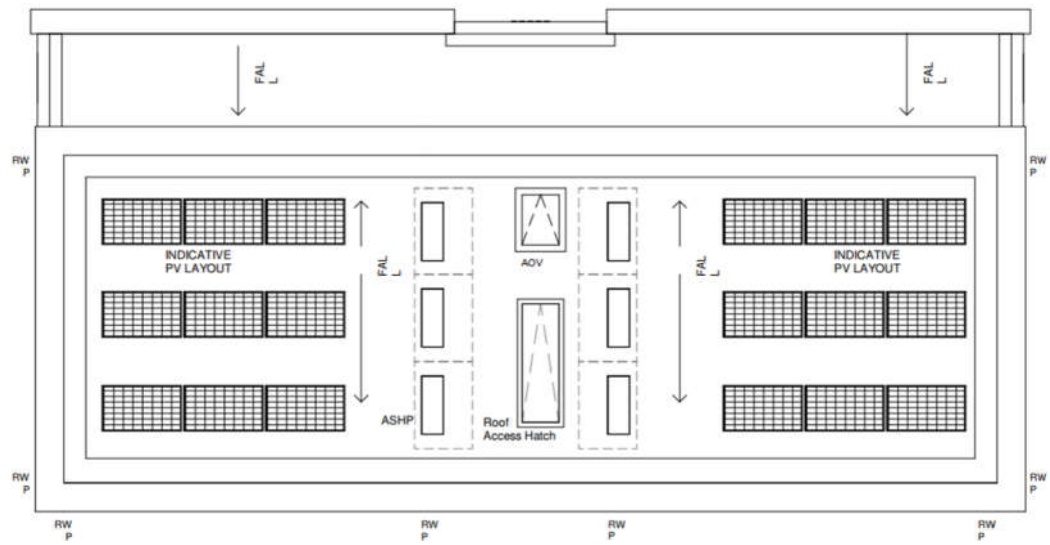
Typical Roof PV layout
