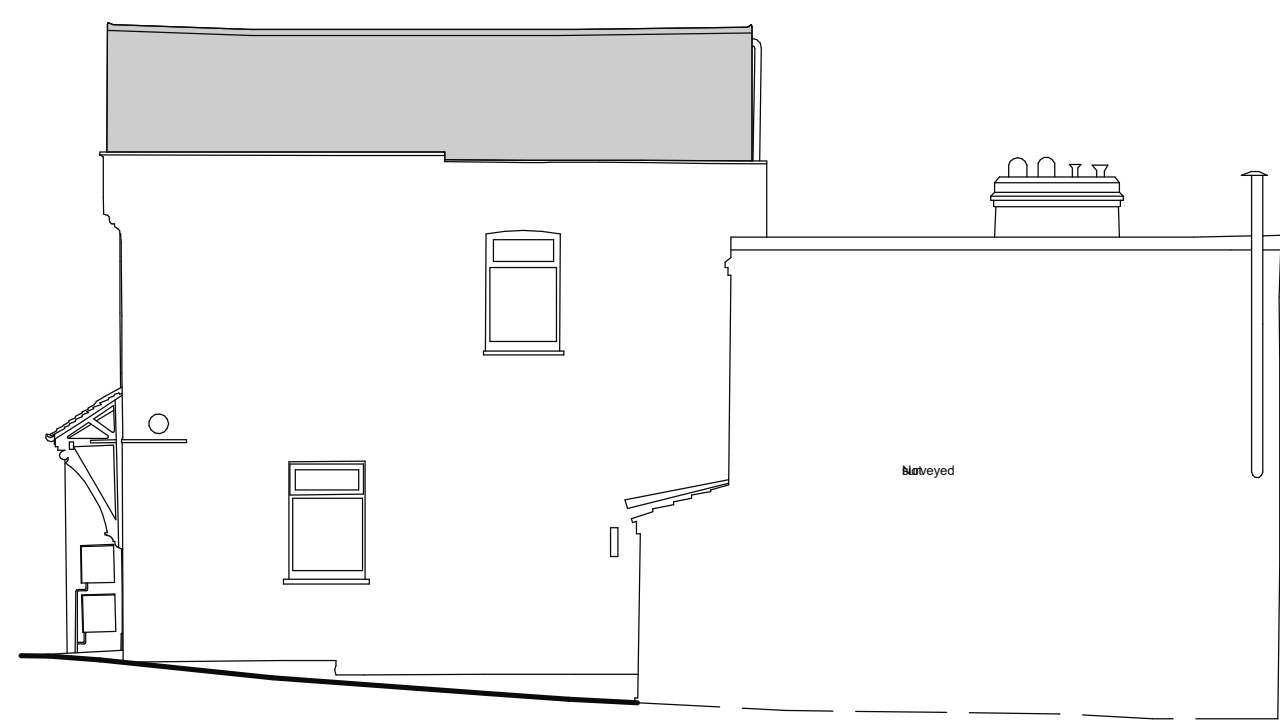
6 PL000 - Existing East Elevation 1 : 100
