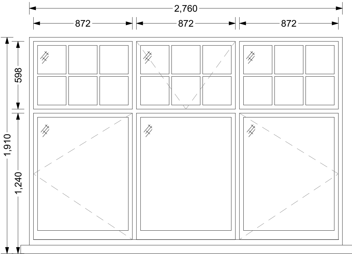
WD-02 Front Elevation
