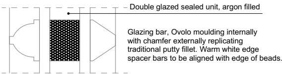
Glazing bar detail 1:2
