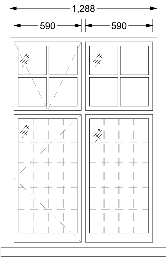
WD-01 Front Elevation
