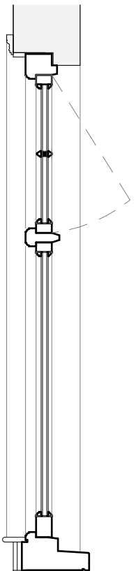
Section Proposed
