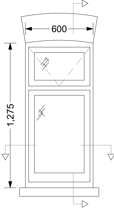
WD-03 Front Elevation
