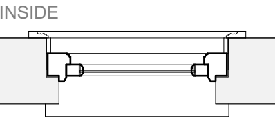
Existing WD-03 Plan
