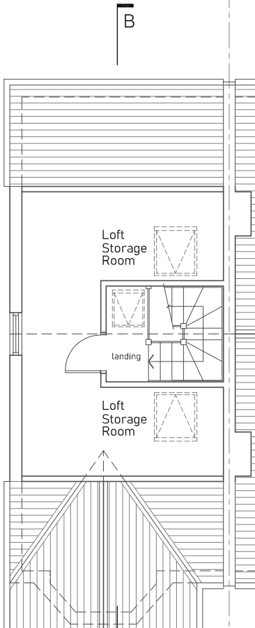
PROPOSED LOFT STORAGE-ROOM PLAN THIRD FLOOR
