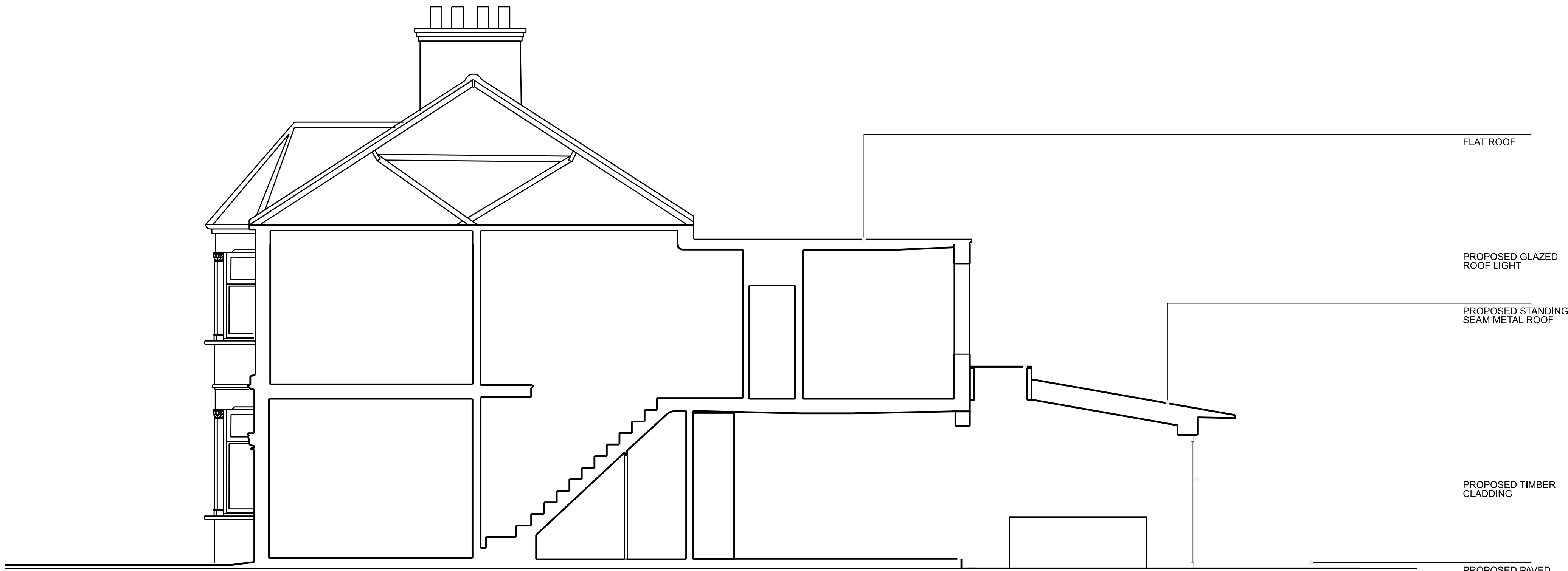
01 SECTION AA SECTION- SCALE 1:50
