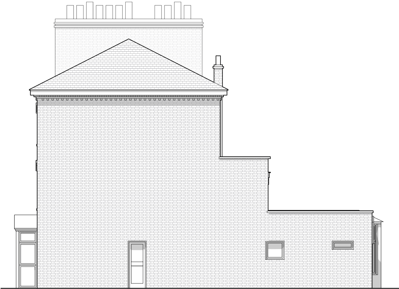
02 - Existing Side Elevation (East) 1:100
