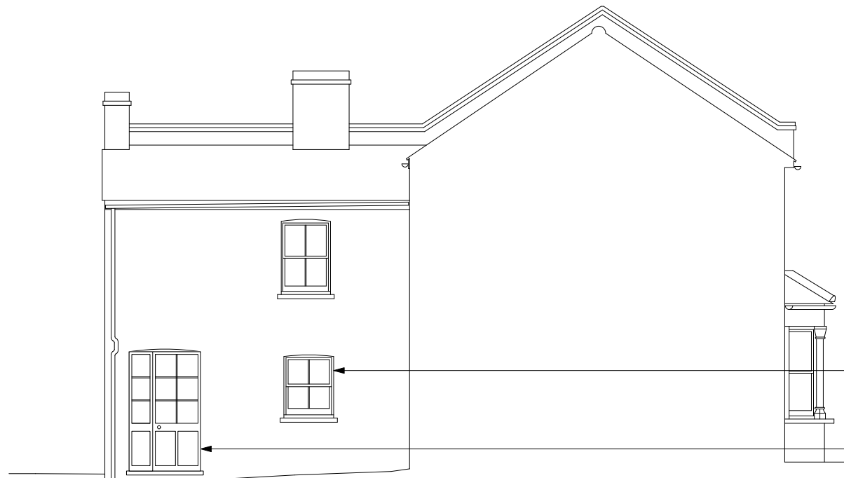
03 Proposed Side Elevation Scale: 1:100
