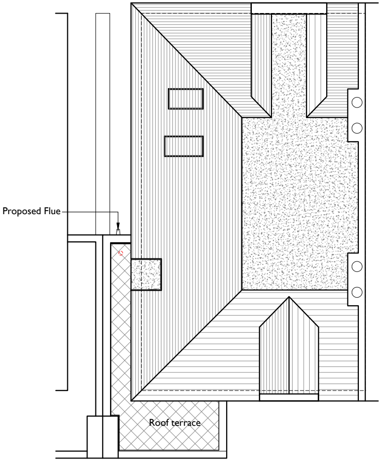
Roof Plan: 1:100 at A3
