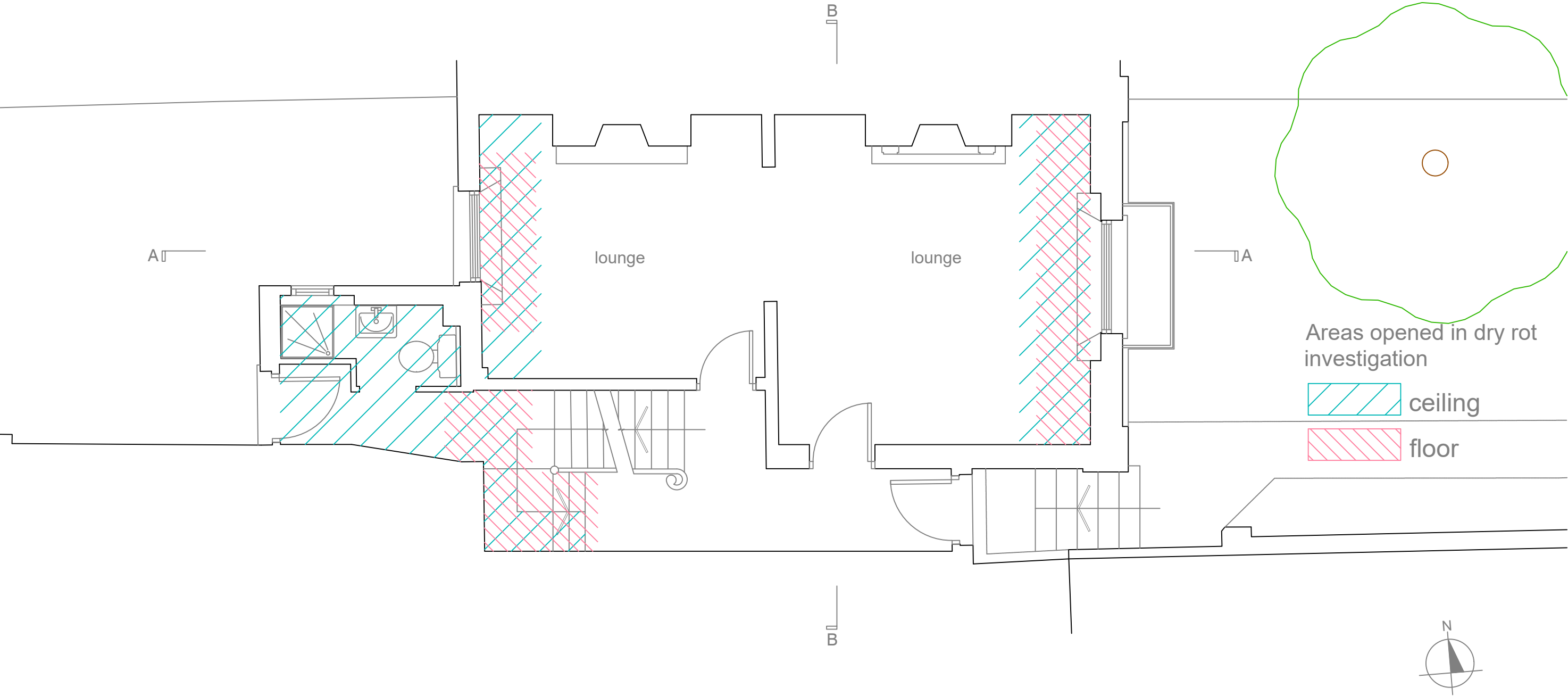
GROUND FLOOR PLAN Measured Survey Drawing
