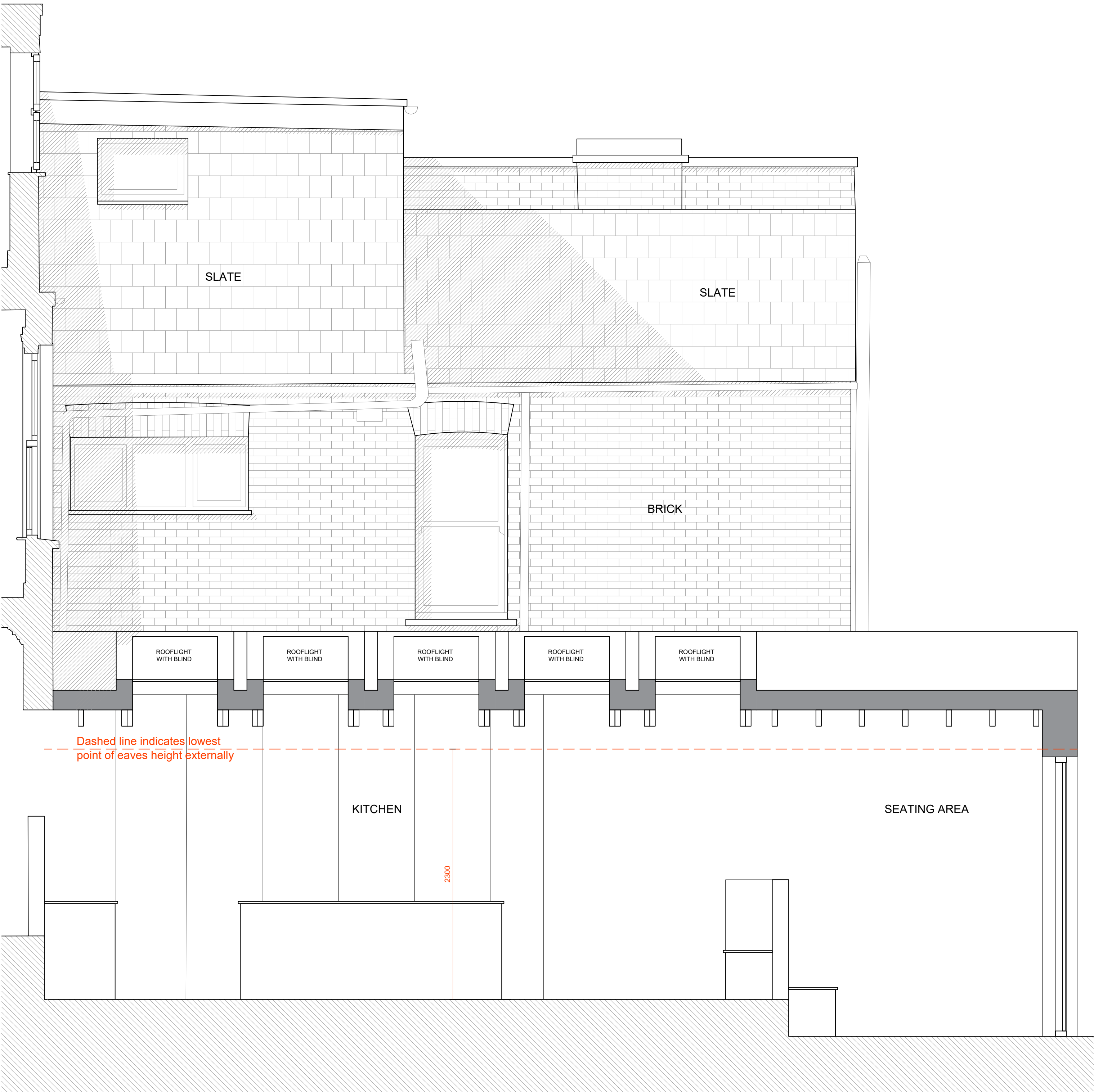
02 Proposed Side Elevation and Section of Extension 1:25@A1 / 1:50@A3
