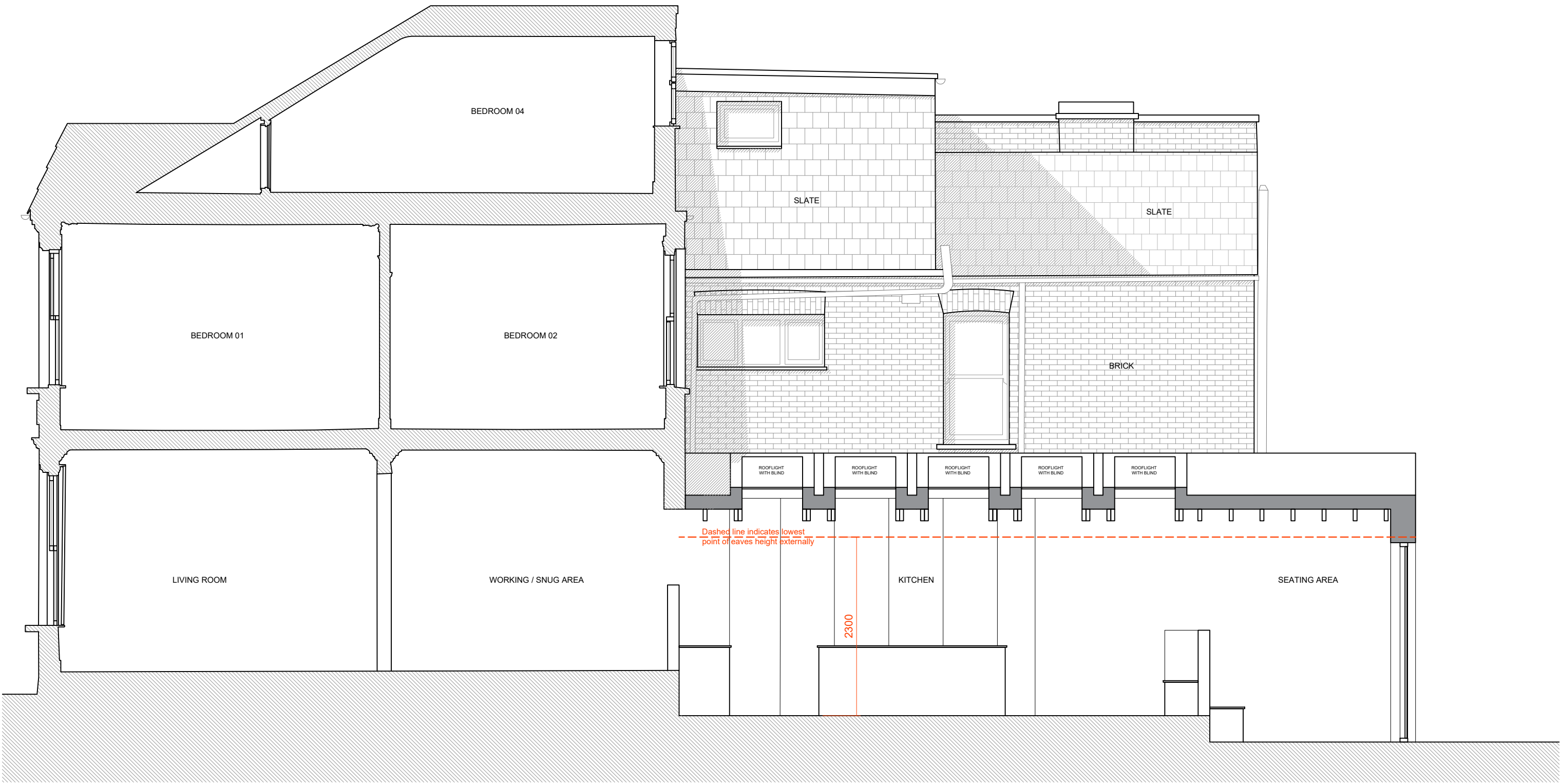
01 Proposed House Section 1:50@A1 / 1:100@A1
