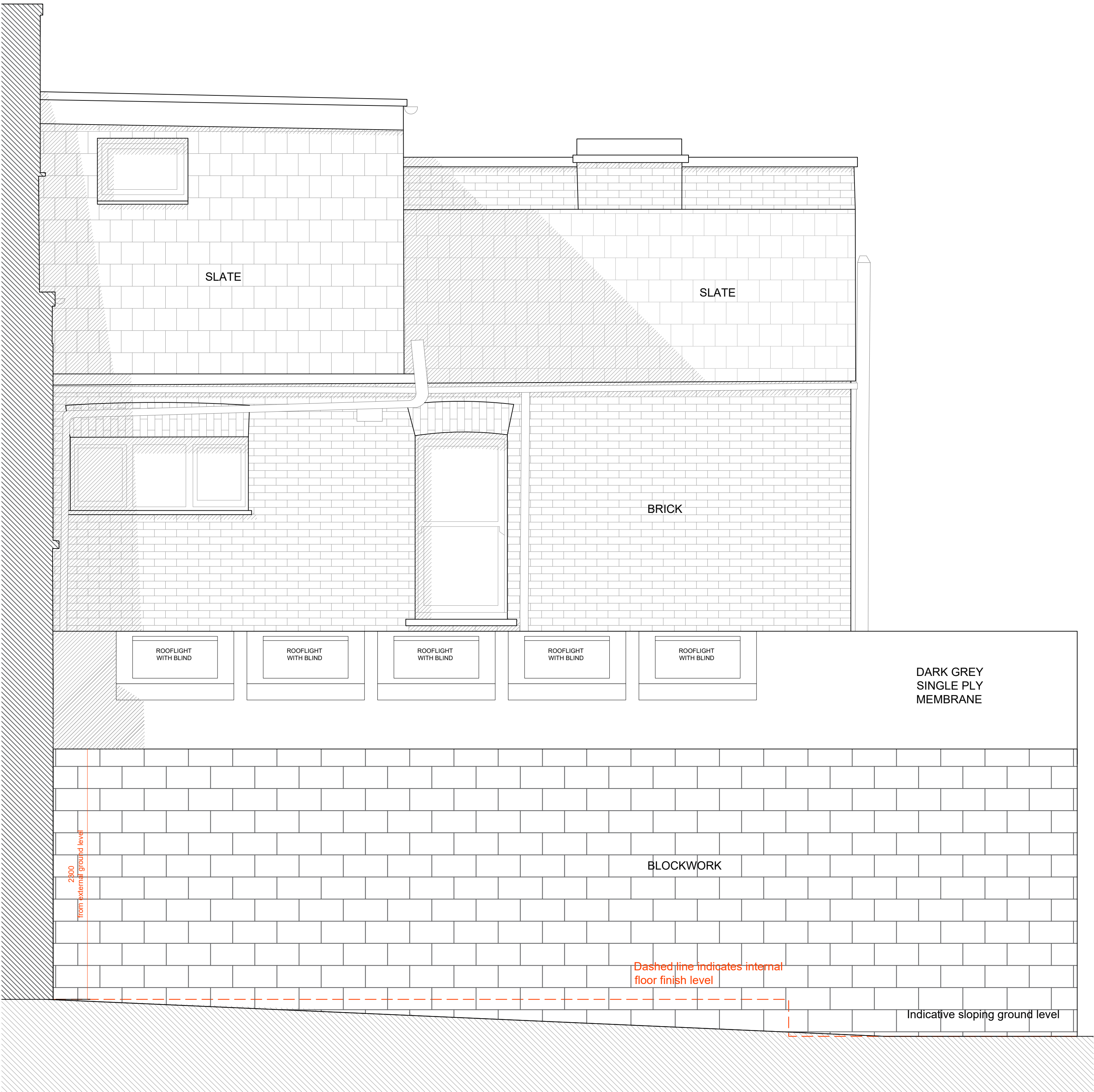
02 Proposed Side Elevation of Extension 1:25@A1 / 1:50@A3
