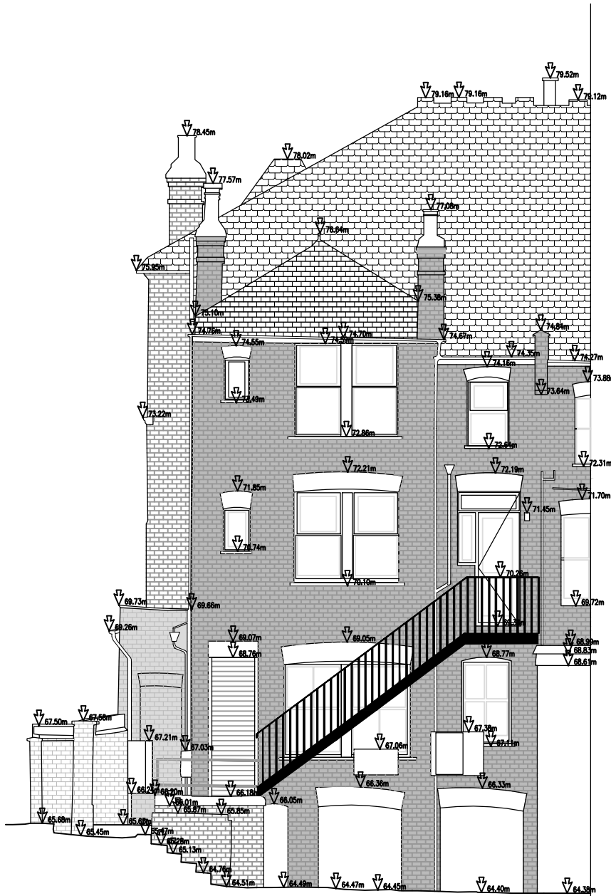
EXISTING ELEVATION 3
