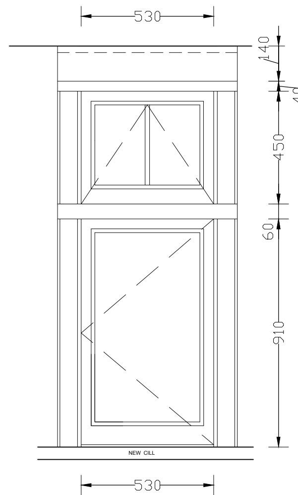
ELEVATION VIEW FROM OUTSIDE 1.W.02
